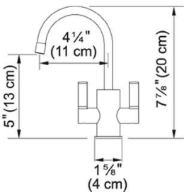
Technical Drawing
