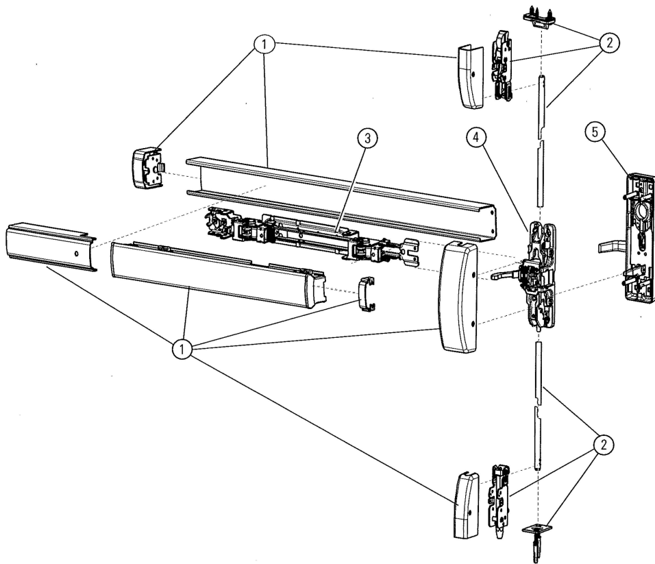
Figure 2.2 2200 Apex Surface Vertical Rod (SVR) Exit Device
